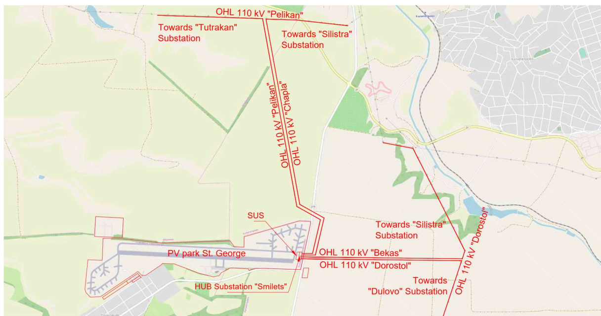
Figure 2. St. George subsites and PV substation and indicative routes of “Pelikan” and “Dorostol” 110kV OHL interruption points
